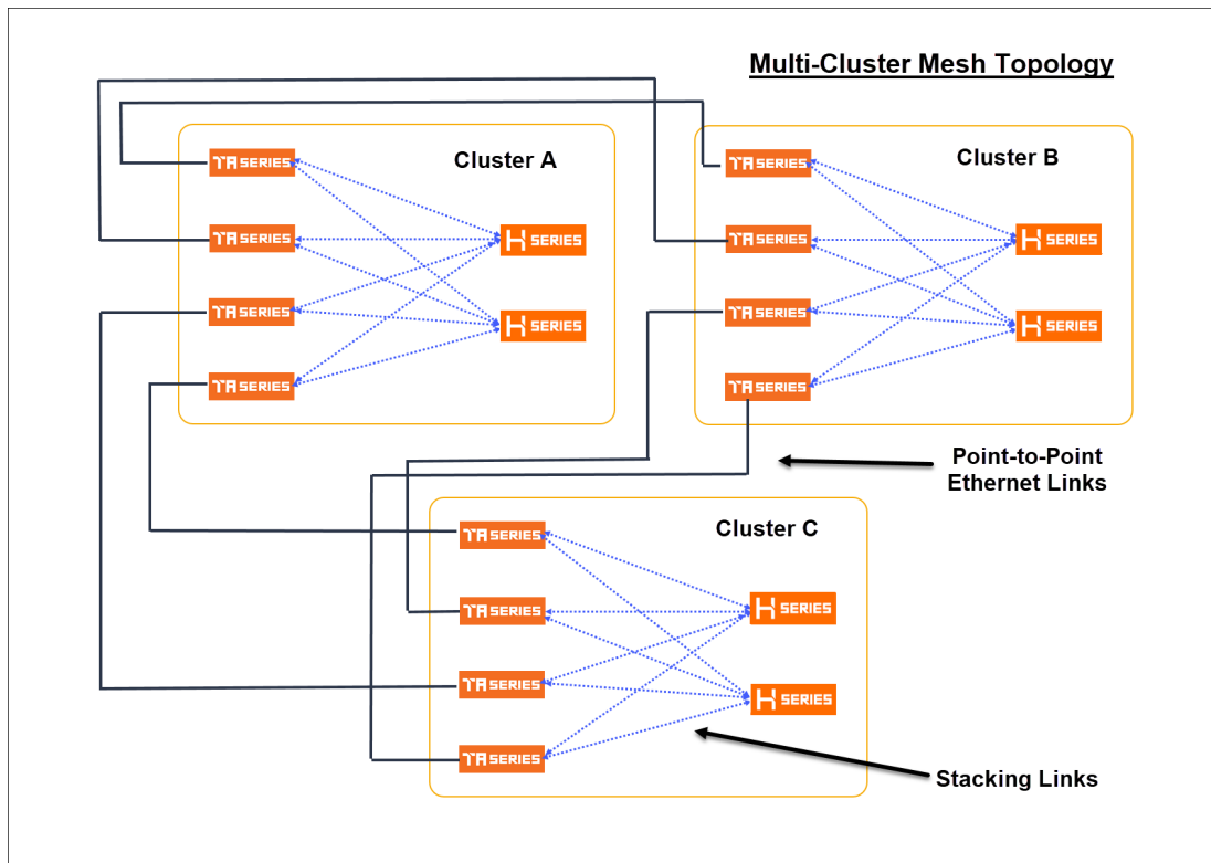
Figure 65 Multi-Cluster Mesh
