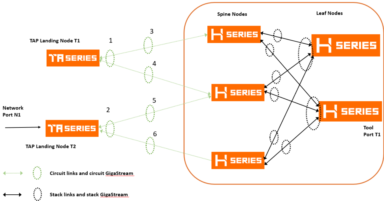
Figure 67 Leaf-Spine Based Topology.
