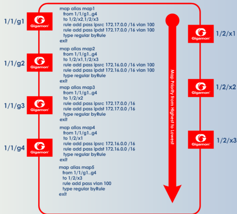
Figure 43 Sending Subnets and VLANs to Different Ports
